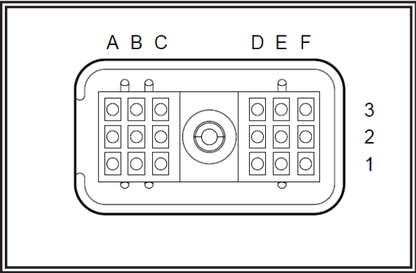
Figure 2 - Delphi Metri-Pack Sealed Connector
