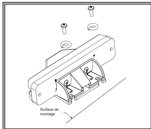
Montage permanent
